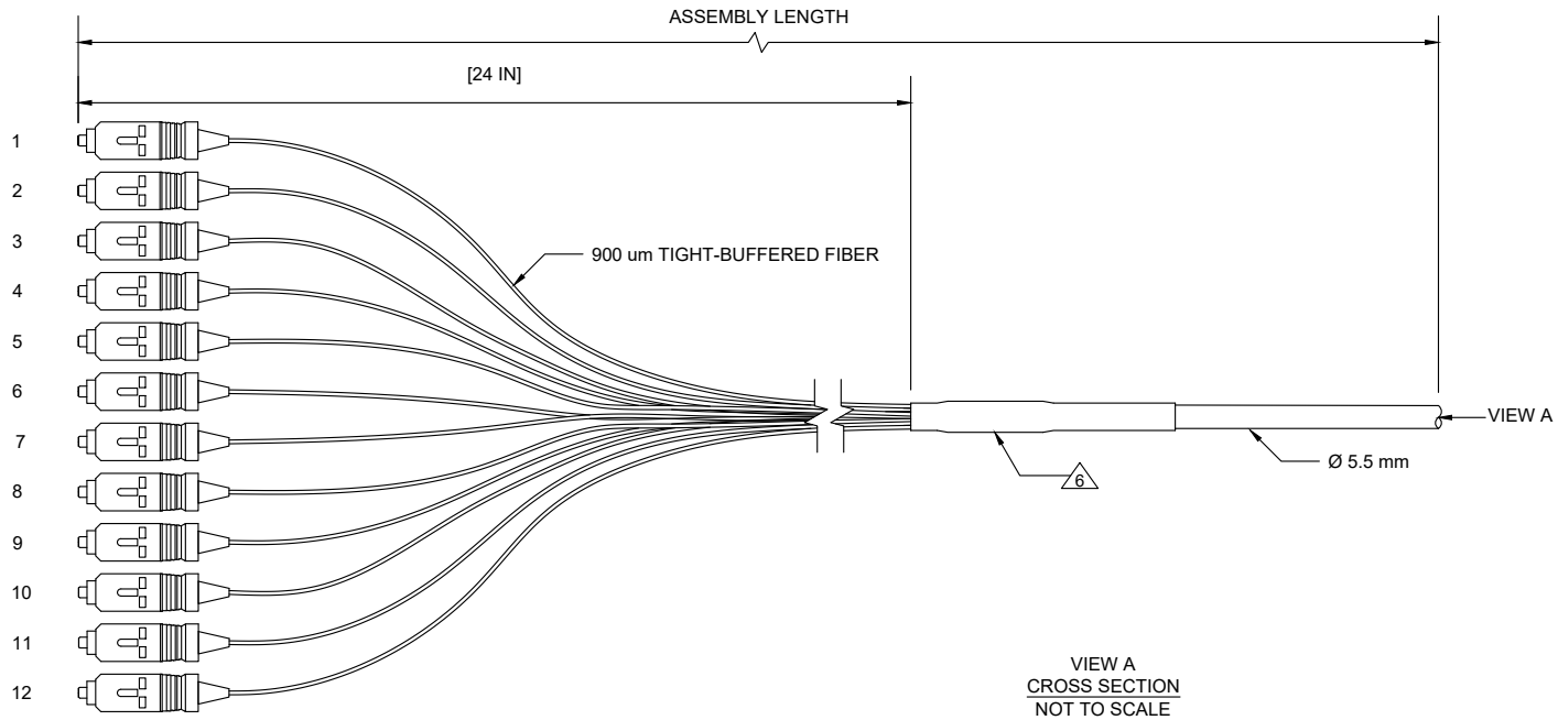
DEPICTION OF PACKAGED ASSEMBLY
